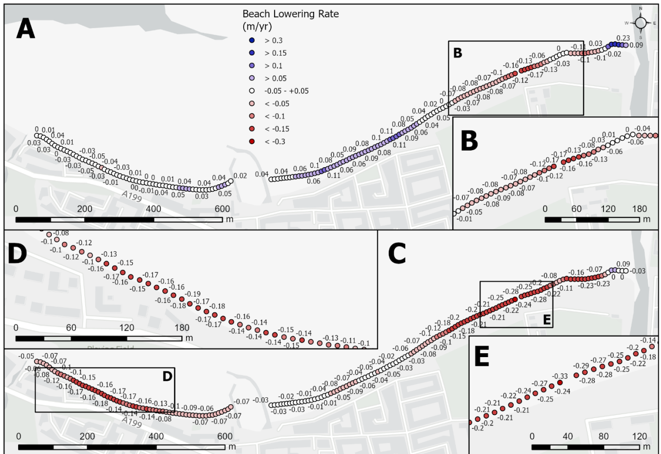
Figure 17: Maps showing a broad estimate of beach lowering based on recent rate of change (between 2018 to 12 th October 2023) and current beach slope (12 th October 2023). Figures 17A & B show the predicted annual rate of beach lowering between 2023 and 2030. Figures 17C-E show the predicted annual rate between 2040 and 2050. Basemap: OS Light Grey via ArcGIS Pro; contains OS data © Crown Copyright and database right 2023. Contains data from OS Zoomstack.
