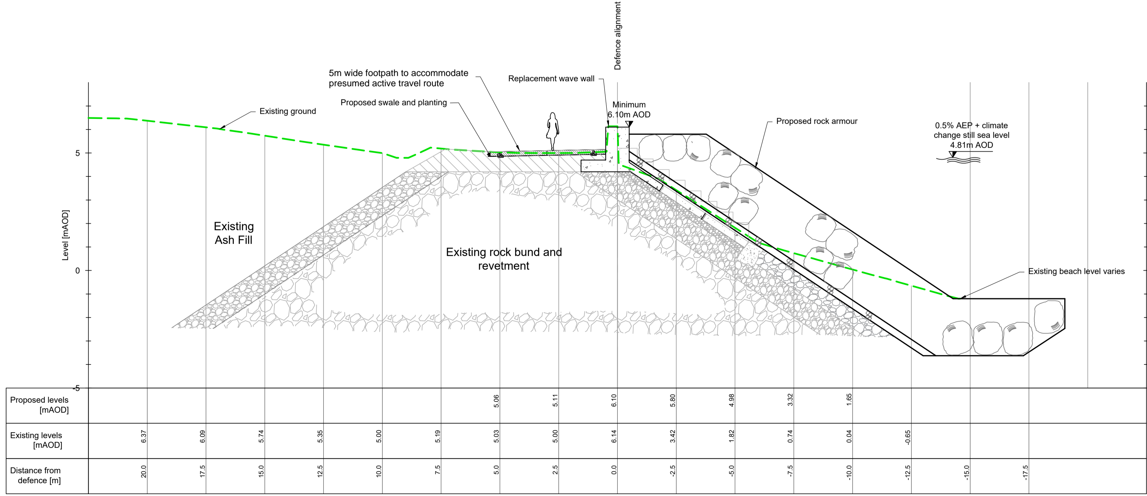
CROSS SECTION I-I SCALE (A1) 1:100 SCALE (A3) 1:200
