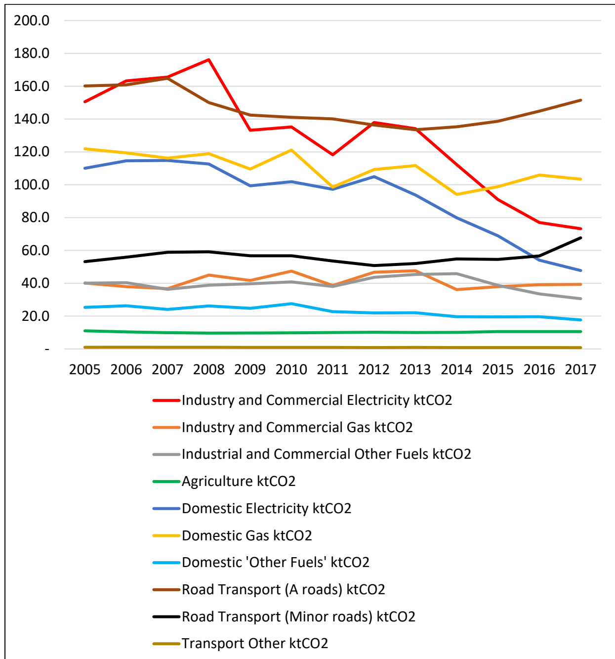
Figure 6: UK Local Authority Carbon Dioxide Emissions Estimates 2005–2017 for East Lothian (kt CO 2 ) 24 within the scope of local authorities: Detailed breakdown of emissions sources by sector:
